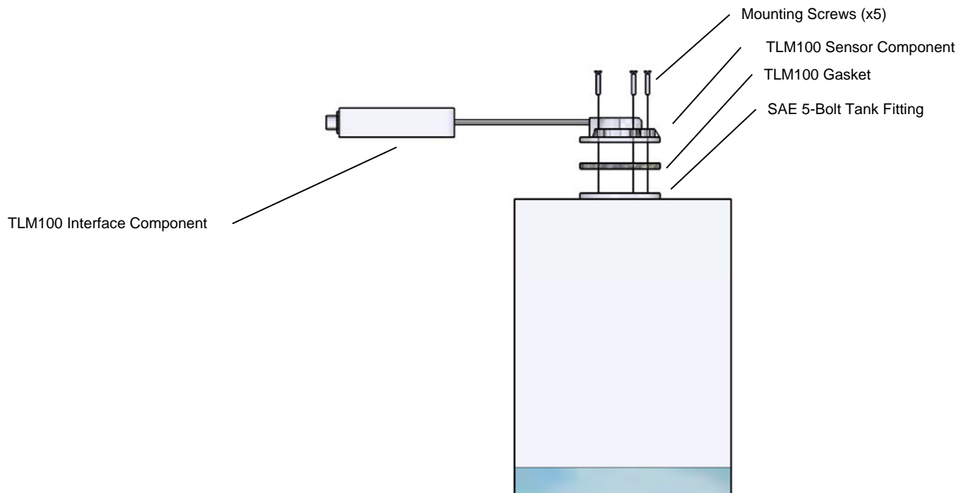
Figure 1 – TLM100 Mounting – SAE 5-Hole Bolt Pattern
